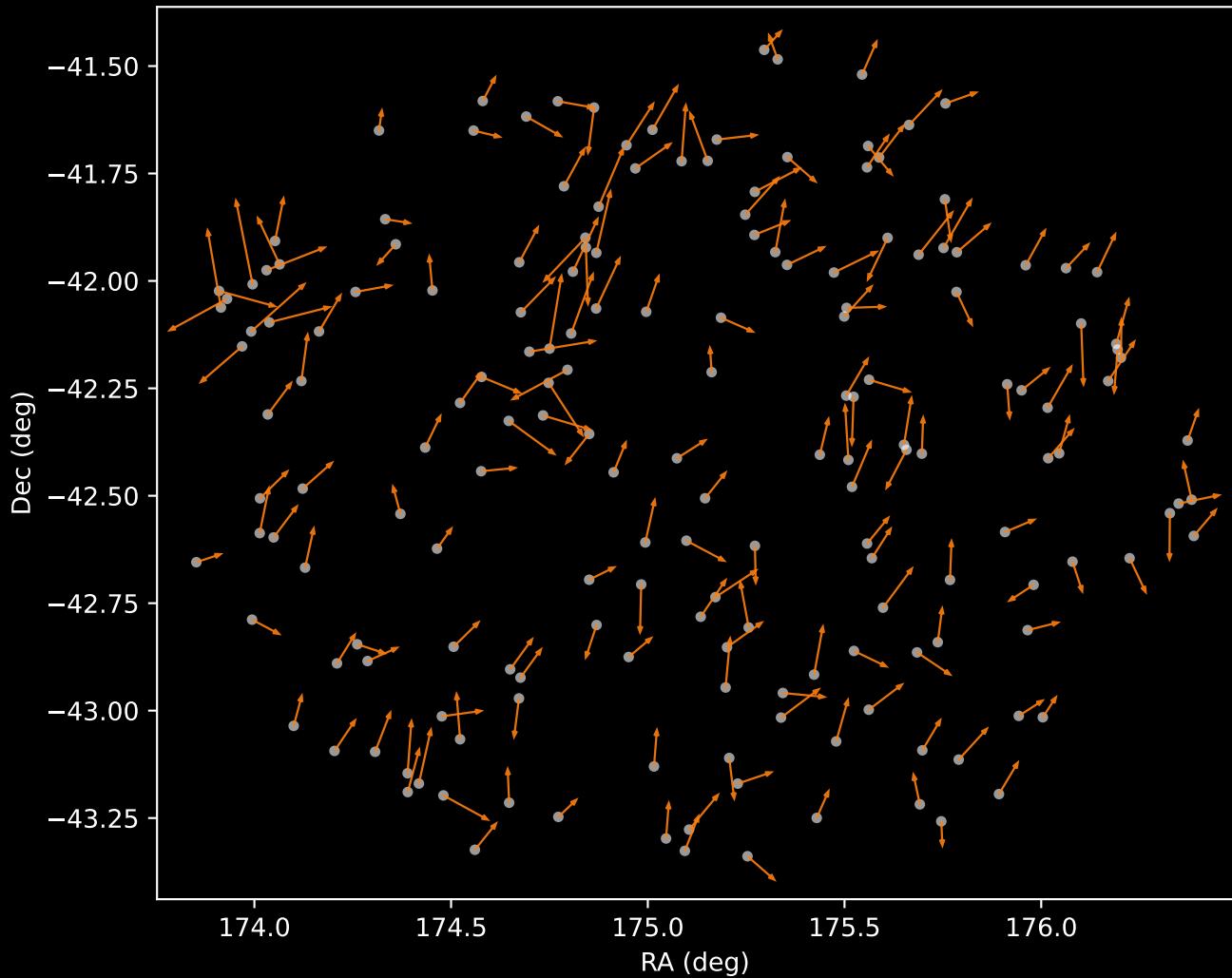
GALAH DR4 Cluster 2 Proper Motion Vectors (n=178)
