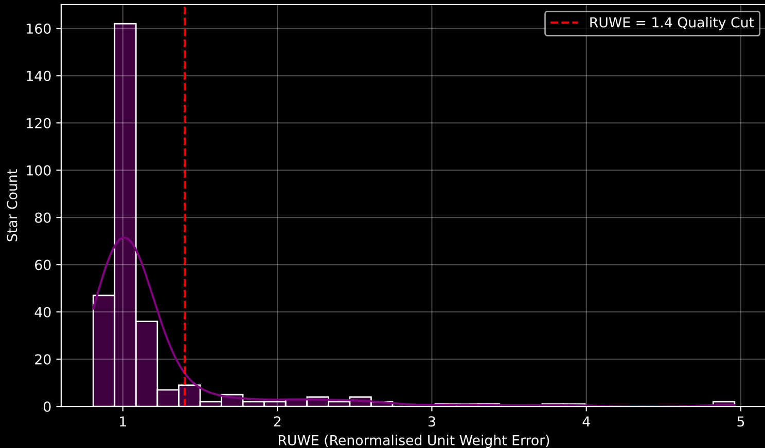
GALAH DR4 Field [363] RUWE Distribution (n= 294)
